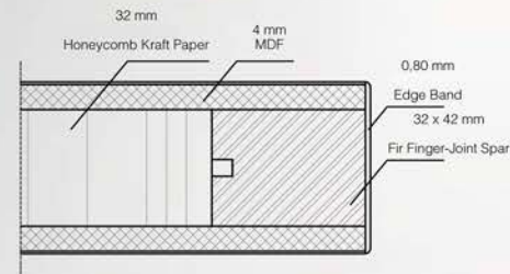
Door Leaf Cross Section
